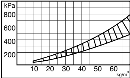
Figure 1: Compressive stress at 10% deformation v density
