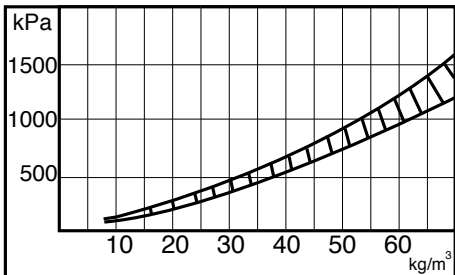
Figure 2: Cross-breaking strength v density
